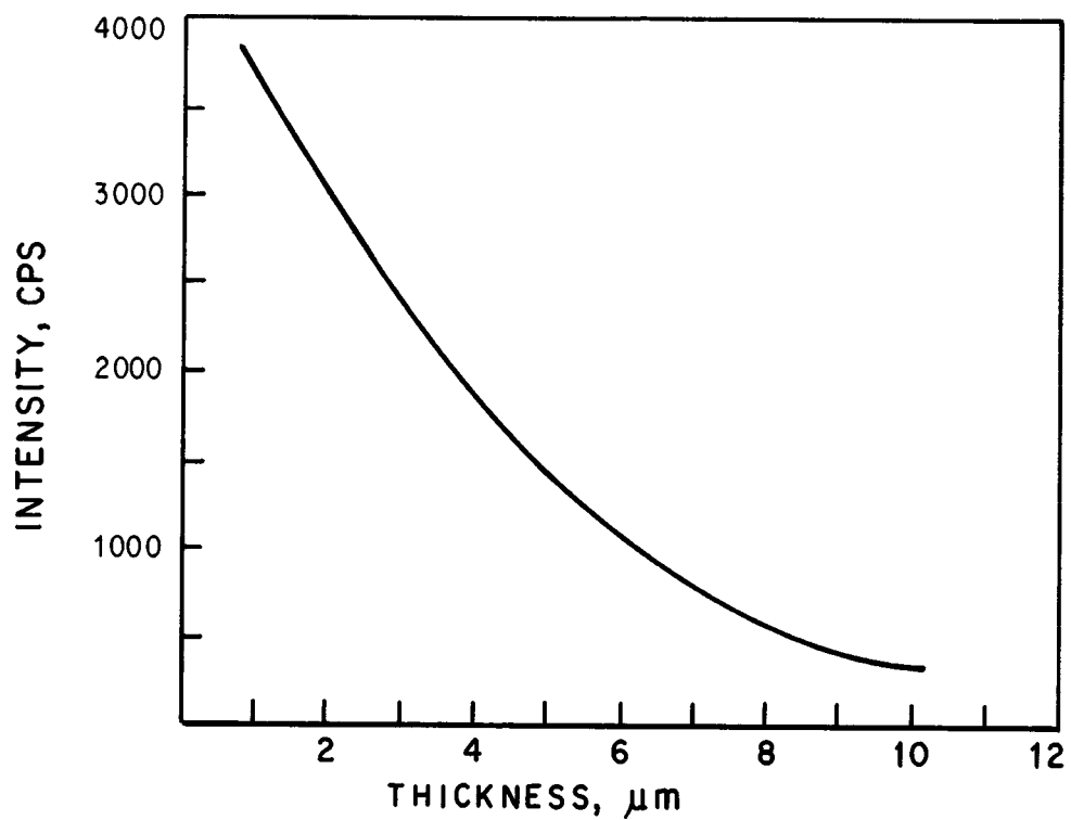
NOTE—Intensity is that of the Cu K\alpha line from the brass substrate after subtraction of background intensity. FIG. X1.2 Calibration Curve for the Determination of a Nickel Thickness by X-Ray Absorption
