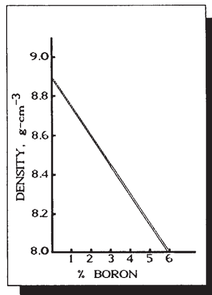
FIG. X1.1 Density of Nickel Coatings with Varying Boron Content
