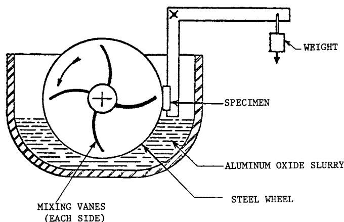
FIG. 1 Schematic Diagram of Abrasive Wear Resistance Apparatus
