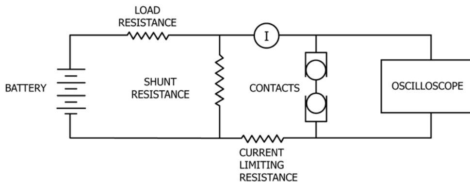
FIG. 1 Circuit Diagram
