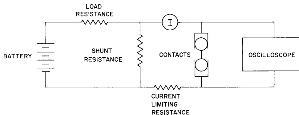
FIG. 1 Circuit Diagram
