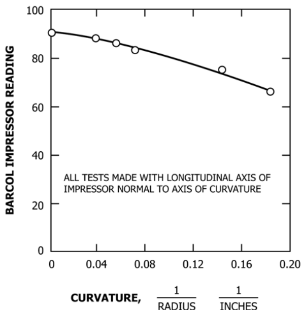
FIG. X1.1 Effect of Curvature of Sheet on Barcol Impressor Readings—Model 934-1, 0.064-in. thick 2024-T3
