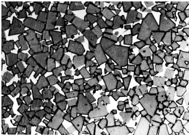
FIG. 2 \alpha Phase (Original Mag. 1500 \times ) (continued)
