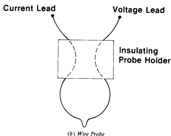
FIG. 1 Arrangement of Current and Voltage Leads to Probe and to Specimen (Typical)
