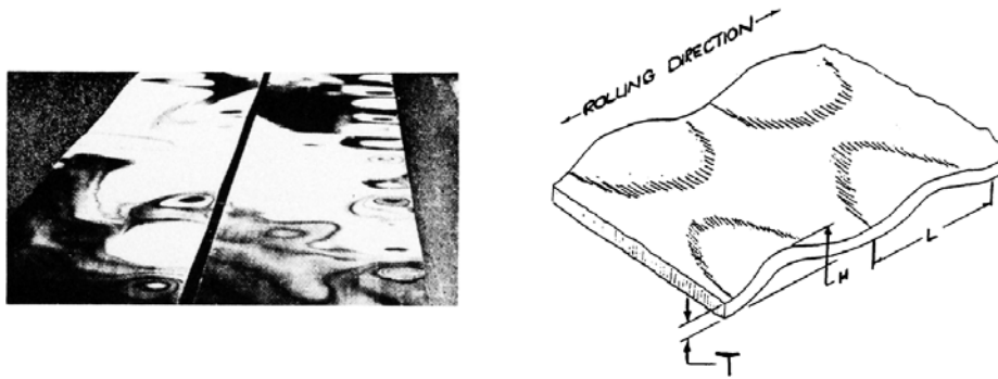
FIG. 2 Wavy Edges
