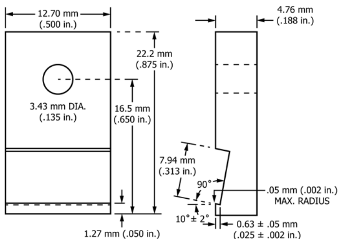
FIG. 4 Grip Design
