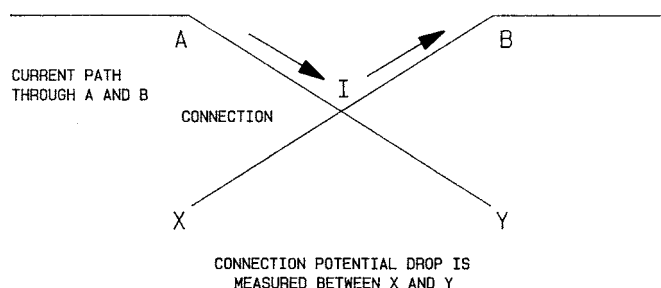
FIG. 1 Four-Wire Method of Measuring Connection Potential Drop
