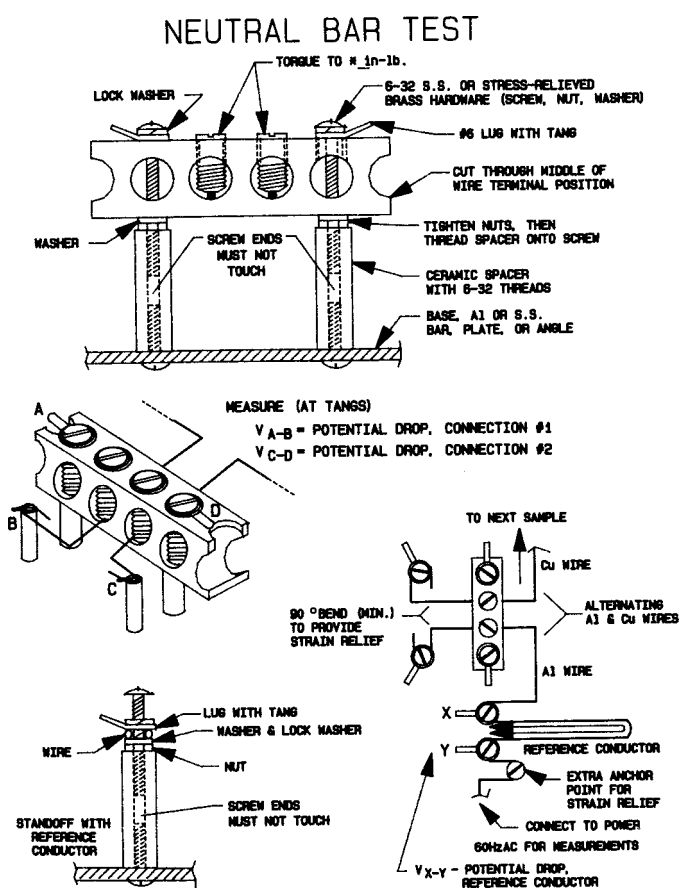
FIG. X1.1 Neutral Bar Test
