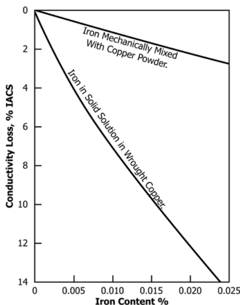
FIG. X2.1 Electrical Conductivity Loss Resulting from Iron Contamination
