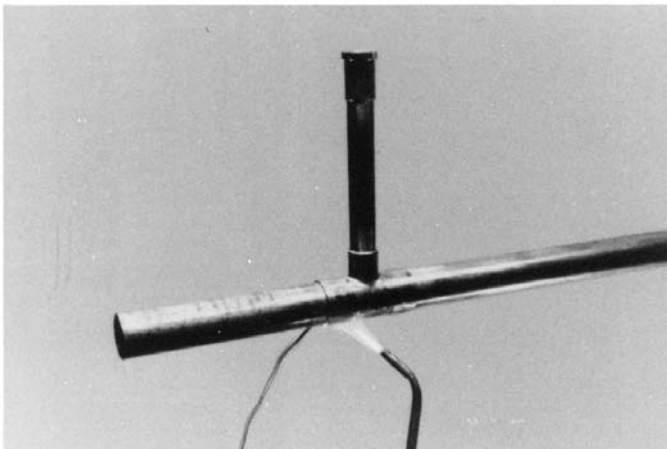
FIG. 19 Soldering
