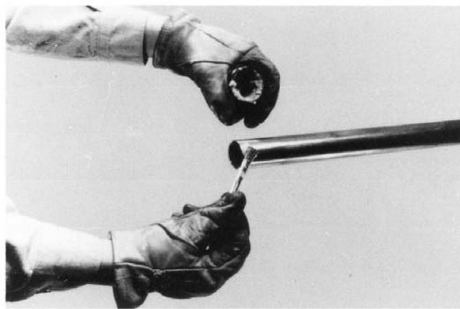
FIG. 10 Fluxing: Tube
