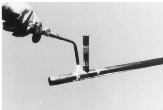
FIG. 16 Preheating: Fitting
