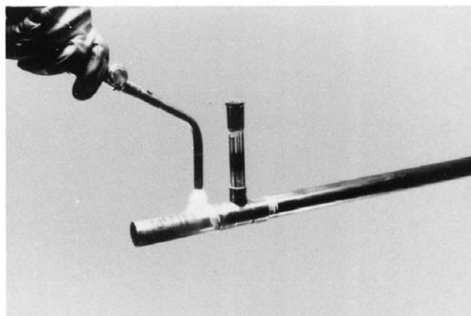
FIG. 15 Preheating: Tube
