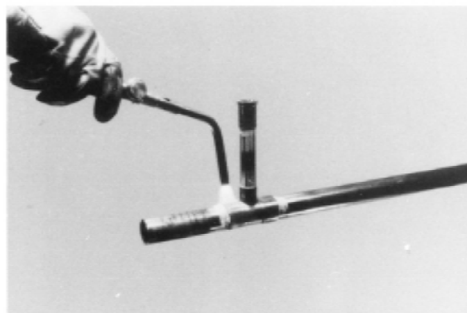
FIG. 16 Preheating: Fitting
