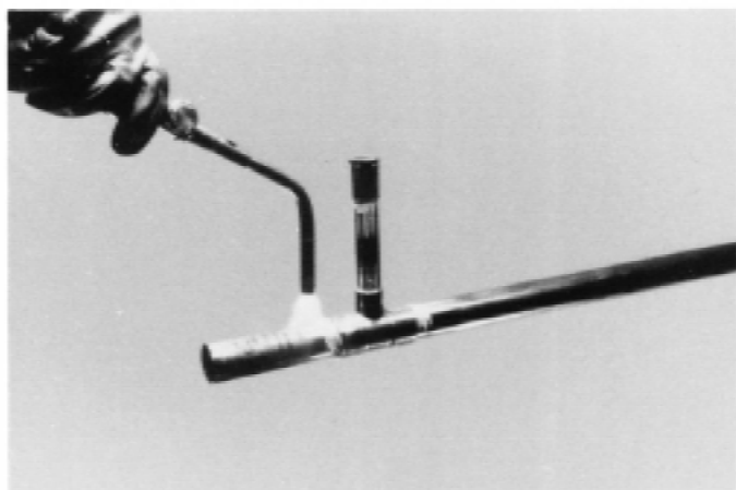
FIG. 15 Preheating: Tube
