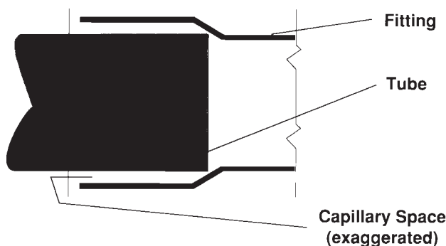
FIG. 14 Desirable Joint Configuration
