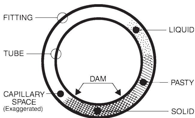
FIG. 20 Schematic of Solder Joint in Horizontal Position
