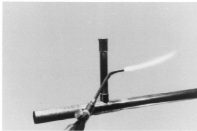
FIG. 17 Heating: Air/Fuel Torch
