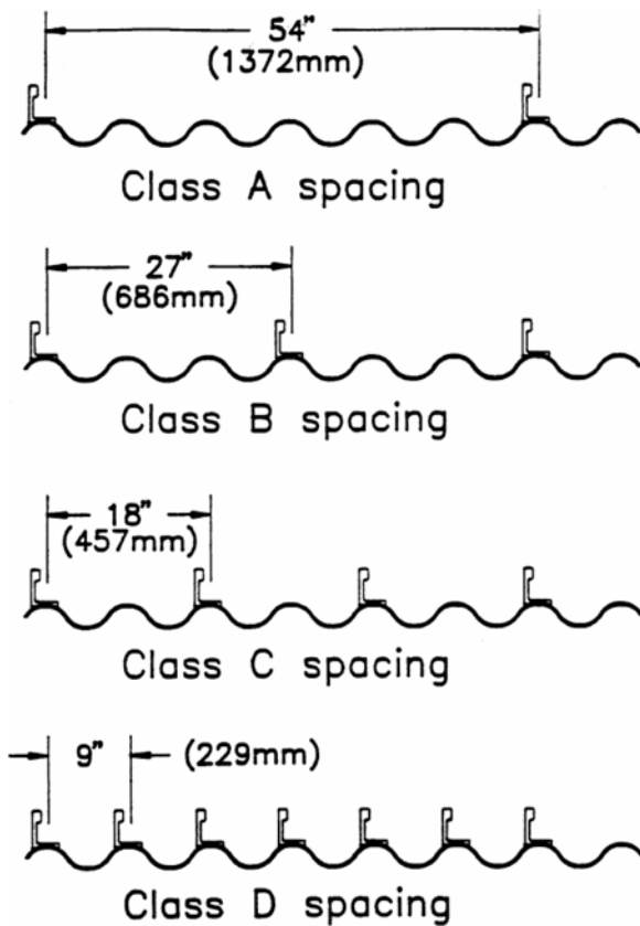
FIG. 4 Rib Stiffener Spacing Classes for Type 1 and Type 2 Ribs
