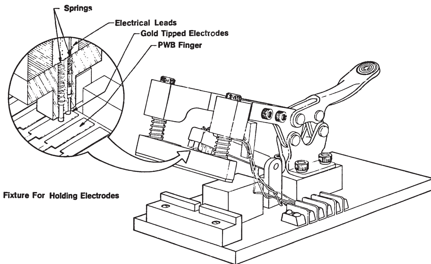
FIG. 1 Resistance Probe
