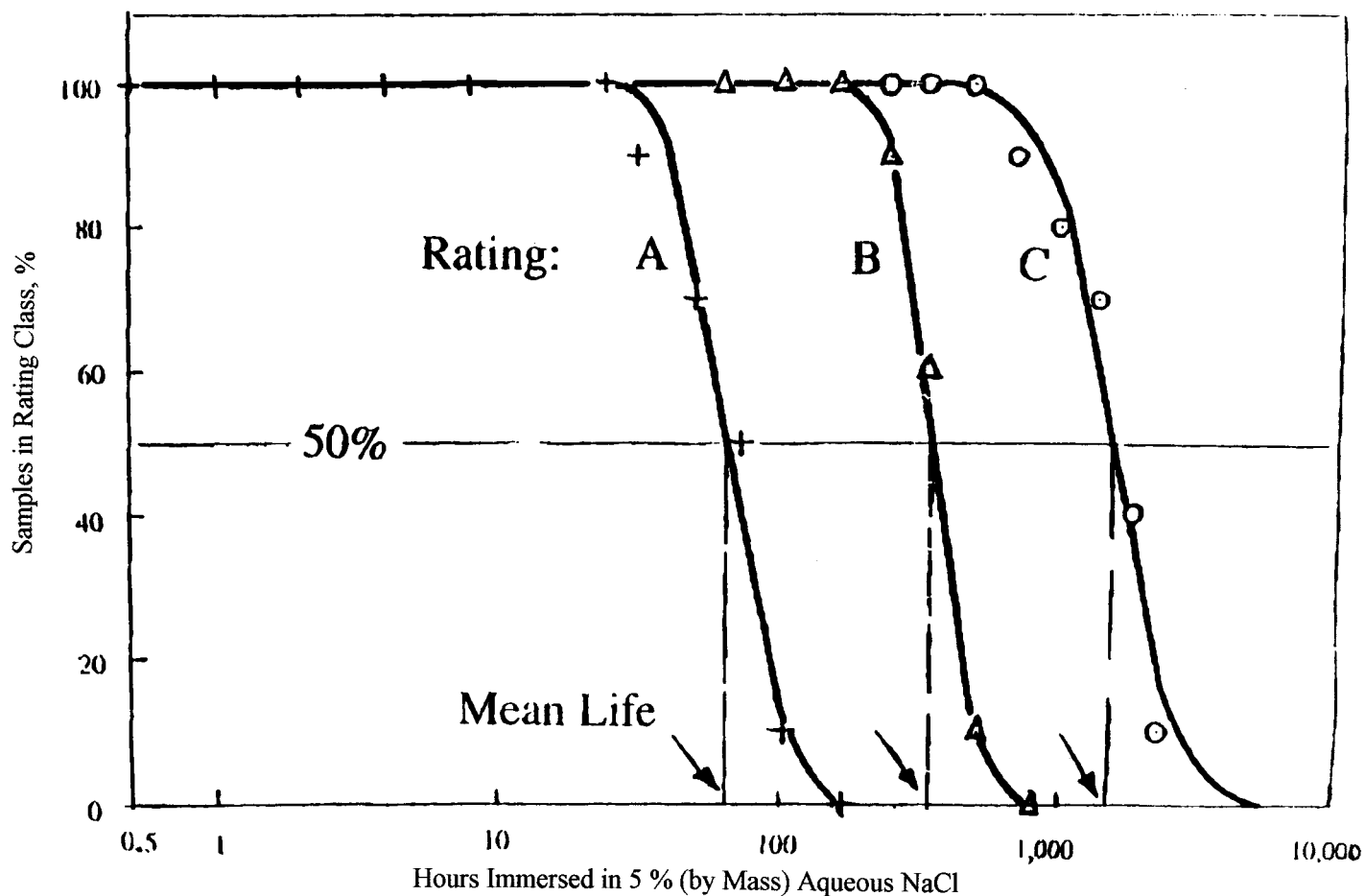
FIG. 2 Plot of Percentage of Replicate Specimens with a Given Rating Versus Immersion Time
