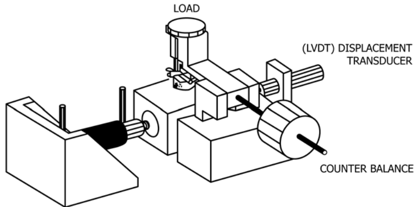
FIG. X2.1 View of a Single Fretting Station
