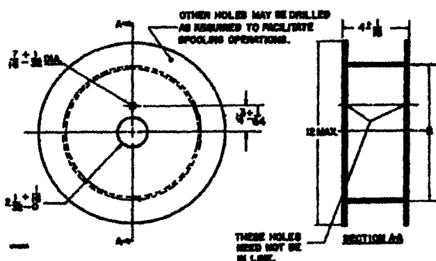
FIG. 15 Typical Wrapped Coiled Round Wire
