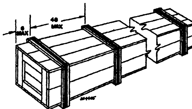
NOTE 1—All dimensions are in inches. FIG. 5 Style 7 Box (Batten Reinforced)
