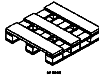
NOTE 1—All dimensions are in inches. FIG. 9 Four-Way Entry TYPICAL PALLET CONSTRUCTION
