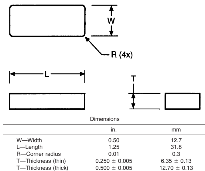
FIG. 2 PM Transverse Rupture Strength Test Specimen
