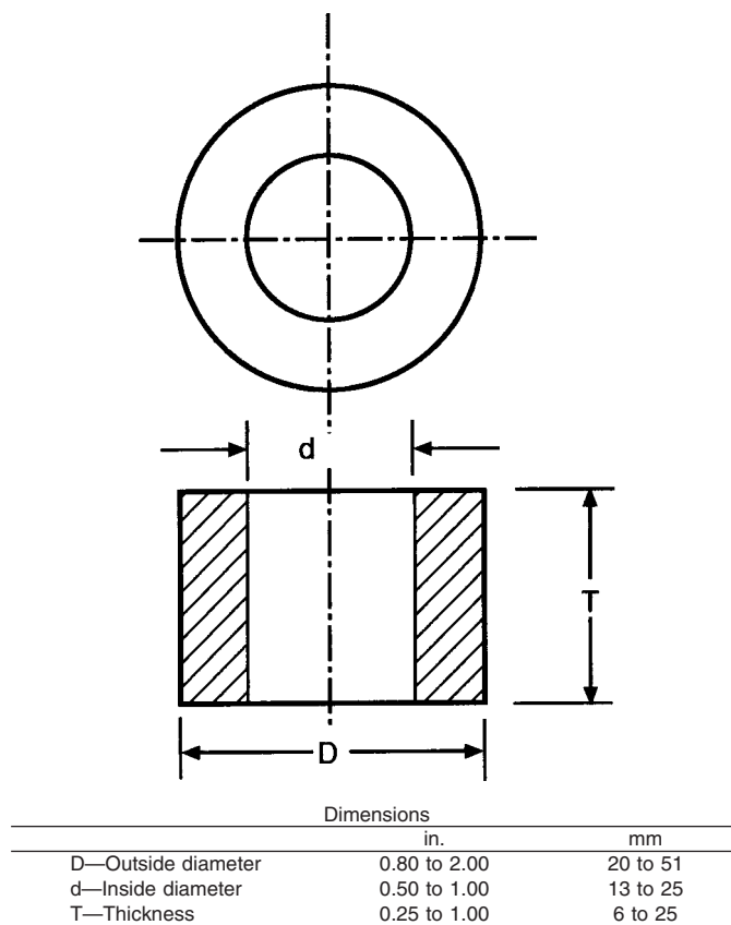
FIG. 3 PM Radial Crushing Strength Test Specimen
