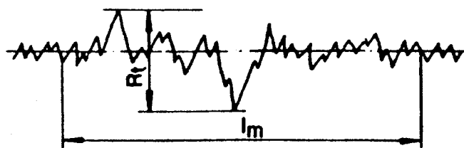
FIG. 2 R_a Arithmetic Mean Roughness Value
