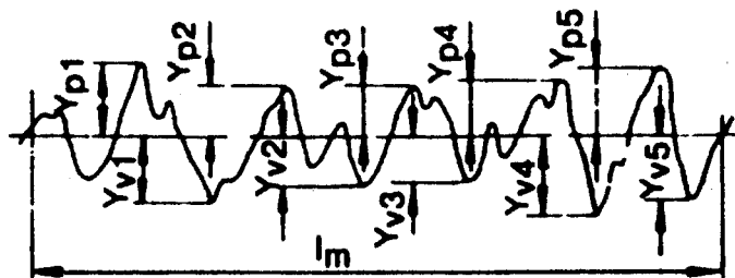
FIG. 4 R_{ZISO} Ten-Point Height
