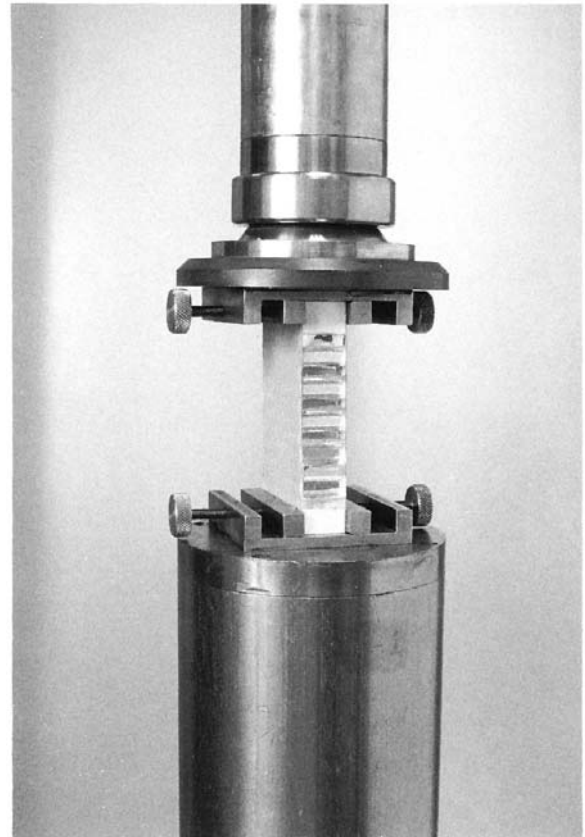
FIG. 1 Edgewise Compression Test Setup
