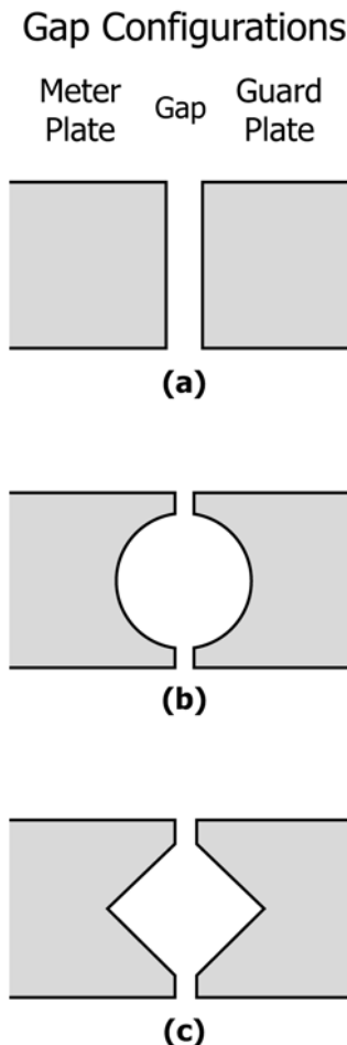
FIG. 2 Designs for the Cross-section of the Gap Between the Meter and Guard Plates
