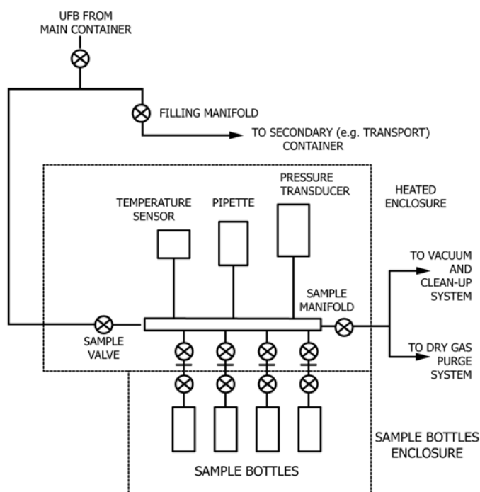
FIG. 2 Schematic Arrangement for Sampling During the Filling of a Transport Container
