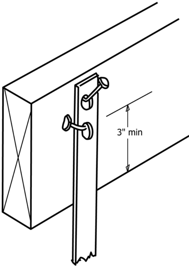
FIG. 7 Flat Hanger Attached to Support Using Nails
