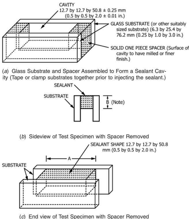
FIG. 1 Sealant Test Specimen
