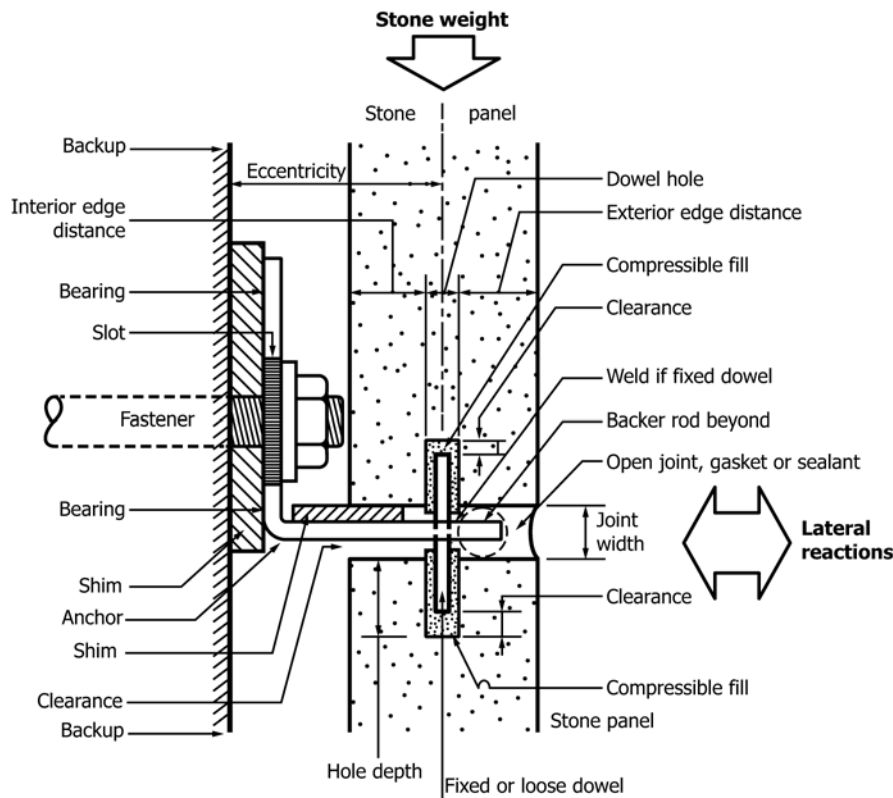
FIG. 8 Dowel Anchor
