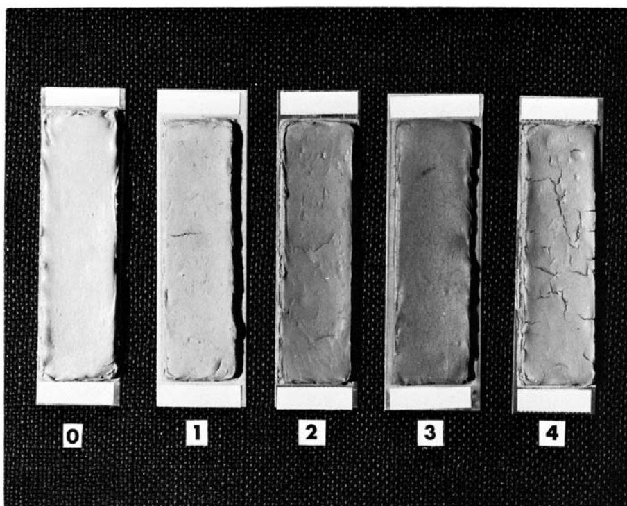
FIG. 1 Examples of Cracking Obtainable in This Test
