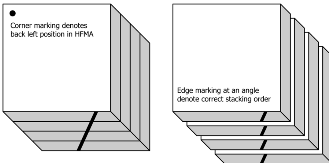
FIG. 3 Examples of Useful Specimen Stack Marking Techniques
