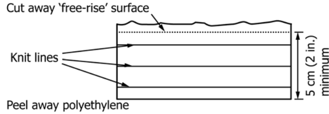
FIG. A2.2 Spray Foam Specimen Preparation
