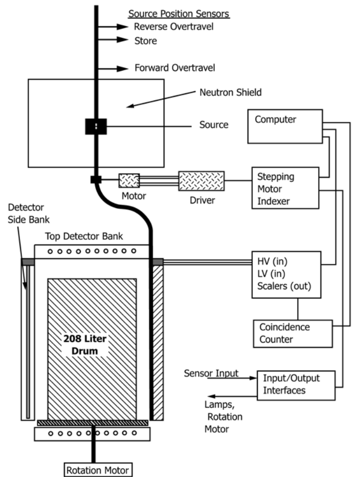
Shuffler Electronic Controls Diagram
