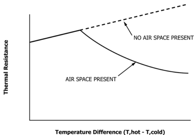
FIG. 1 Schematic of Thermal Resistance for a Permeable Attic Insulation Under Simulated Winter Conditions (Heat Flow Up)
