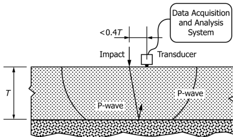
FIG. 4 Schematic of Testing Configuration for Impact-Echo Test (Procedure B)
