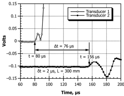
FIG. 3 Example of waveforms obtained using Procedure A (Only Early Part of Waveforms are Plotted)
