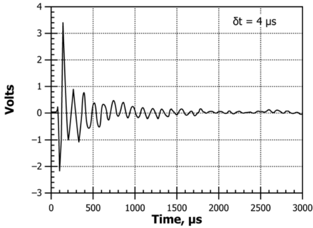
FIG. 5 Waveform and Amplitude Spectrum for a Valid Impact-Echo Test of 250-mm Thick Concrete Slab
