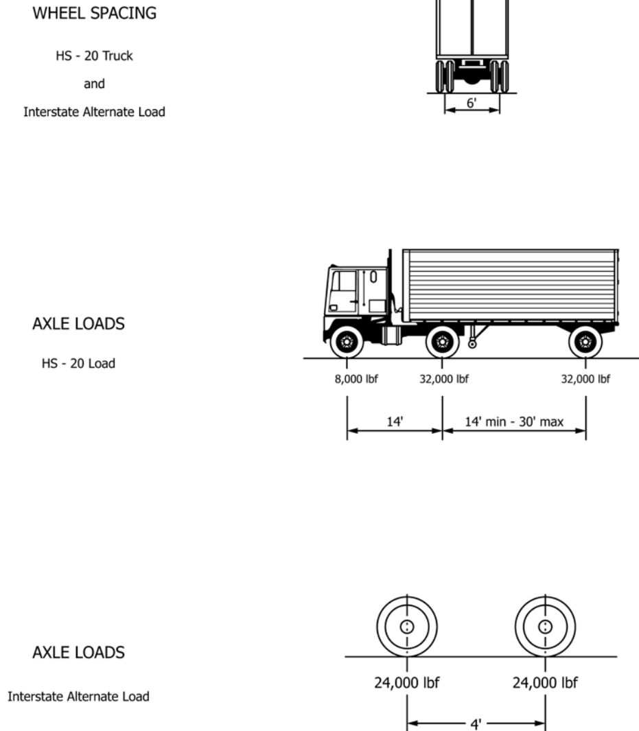
FIG. X1.1 Axle Loads for Box Section Standard Designs
