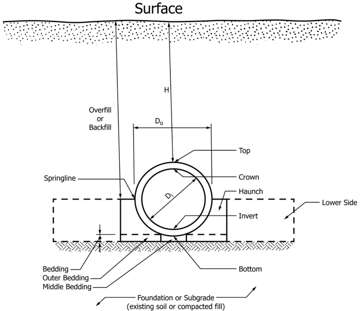
FIG. 1 Pipe/Installation Terminology
