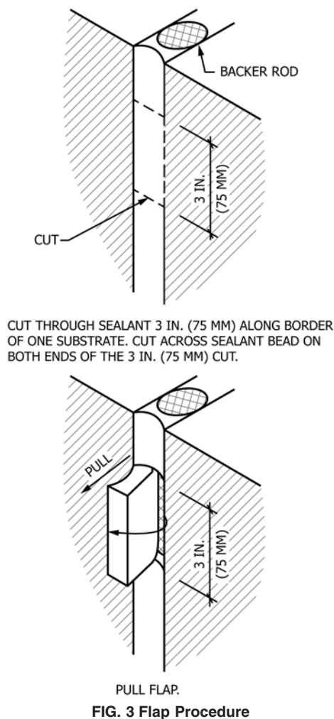
FIG. 3 Flap Procedure
