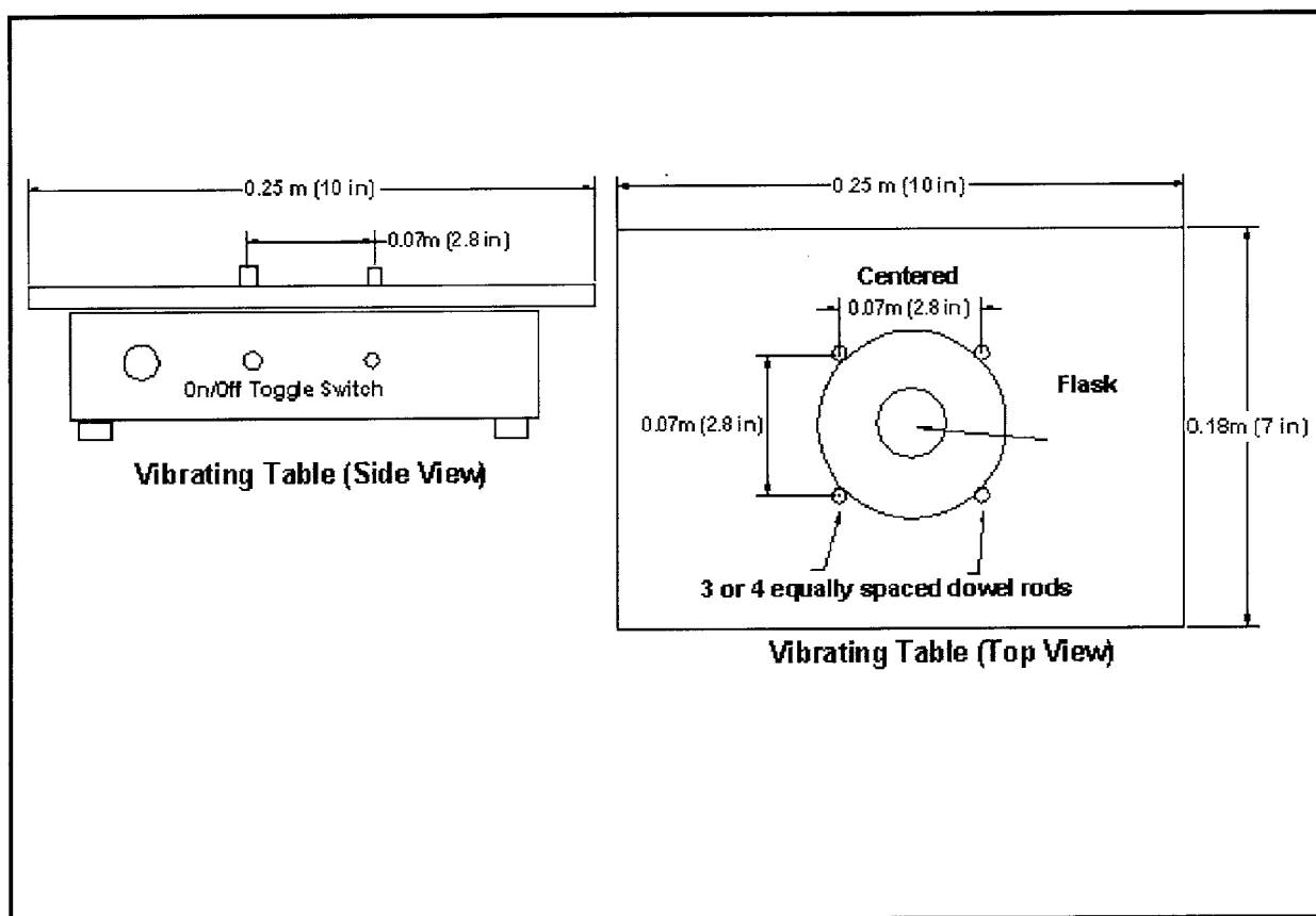
FIG. 1 Vibrating Table
