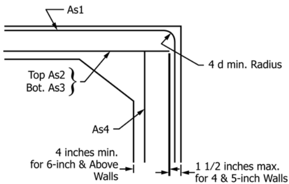
FIG. 3 Detail Inner Reinforcement
