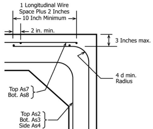
FIG. 6 Detail Option
