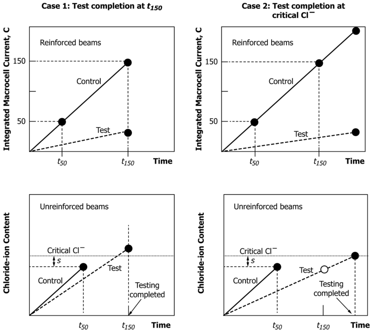
FIG. X1.1 Schematic to Illustrate when Corrosion Testing is Completed and to Illustrate the Required Performance in Terms of Integrated Macrocell Current
