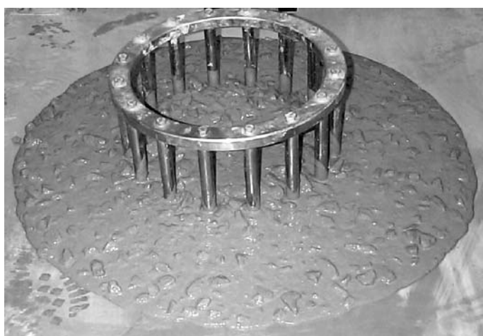
FIG. 3 J-Ring Flow
