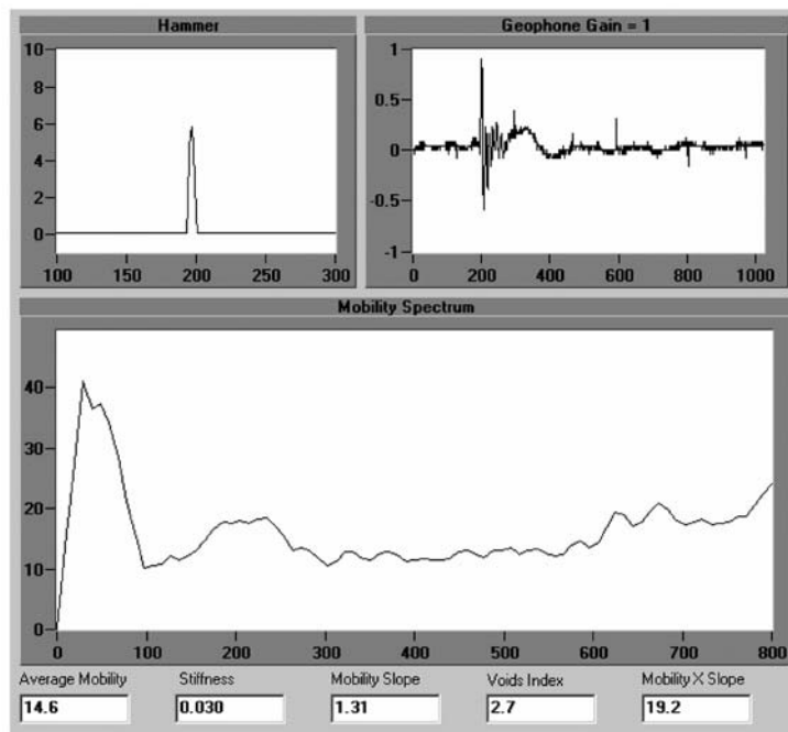
FIG. 5 Invalid Waveform (Upper Right Plot) Caused by Movement of the Velocity Transducer Base
