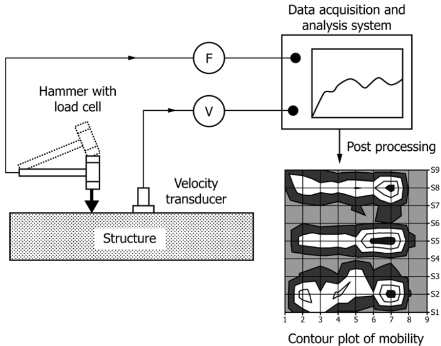
FIG. 1 Schematic of the Test Set-Up and Apparatus for Impulse-Response Test
