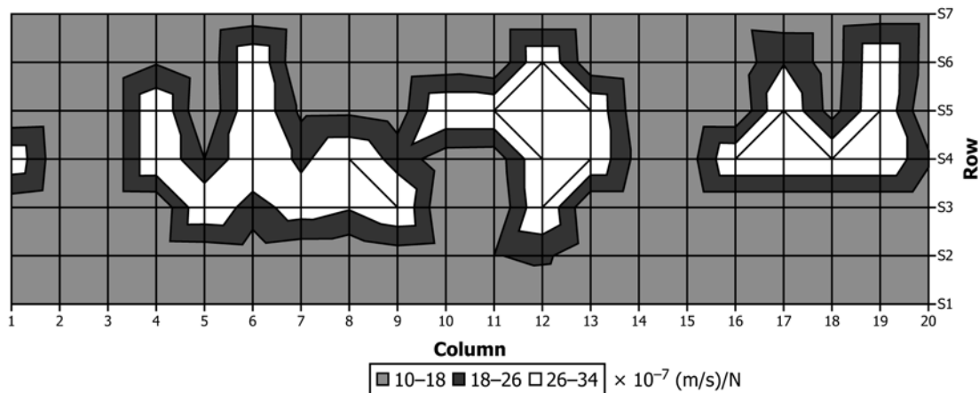
FIG. 6 Typical Contour Plot of Average Mobility (White Regions Indicate Higher Mobility)
