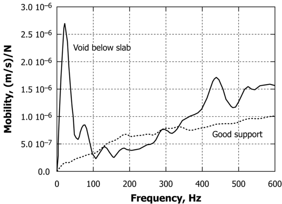
FIG. X1.3 Example of Mobility Spectrum for Test on Slab-on-Ground with Void Below Slab Compared with Test at Point Without Void
