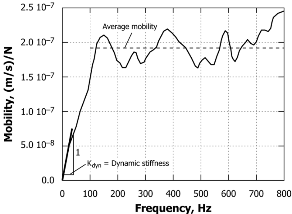
FIG. 3 Example of a Mobility Spectrum Obtained from an Impulse Response Test of a Plate-Like Concrete Element
