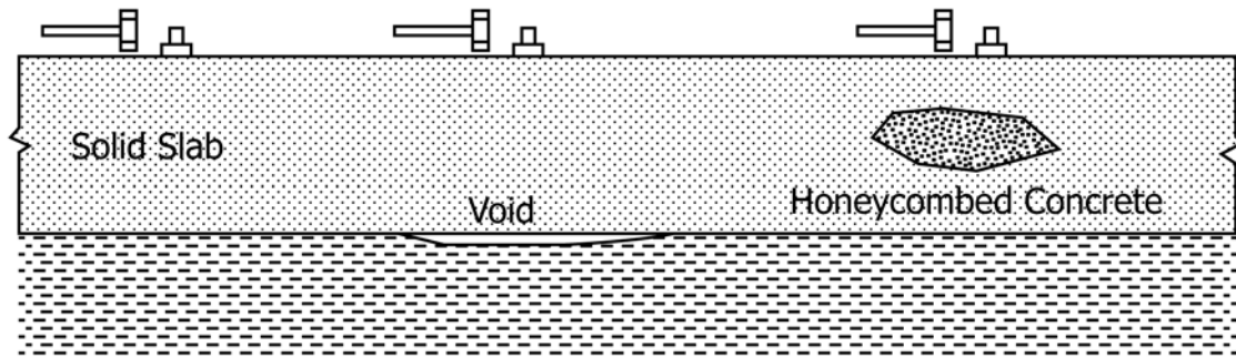
FIG. X1.1 Example of Slab-on-Ground with Different Types of Defects
