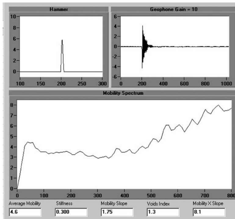
FIG. 4 Valid Set of Waveforms for Hammer Voltage Versus Time and Velocity Transducer Voltage Versus Time (Mobility Spectrum is at Bottom)
