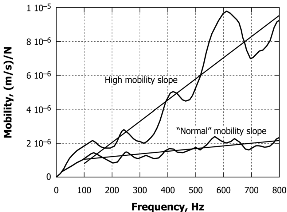
FIG. X1.2 Example of Steep Mobility Spectrum at a Test Point with Poor Consolidation Compared with Spectrum at Point with Sound Concrete
