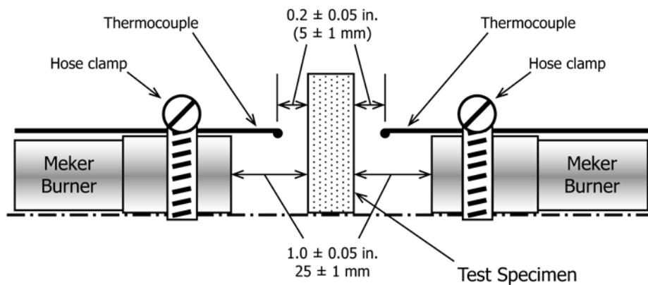
FIG. 3 Alignment of Burners and Thermocouples with Respect to Test Specimen
