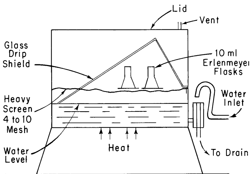
FIG. X6.1 Steam Chamber
