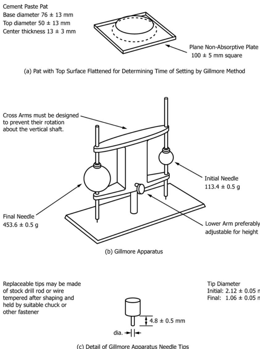
FIG. 1 Gillmore Apparatus and Test Specimen
