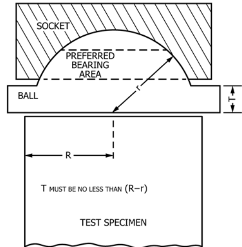
FIG. 1 Schematic Sketch of a Typical Spherical Bearing Block
