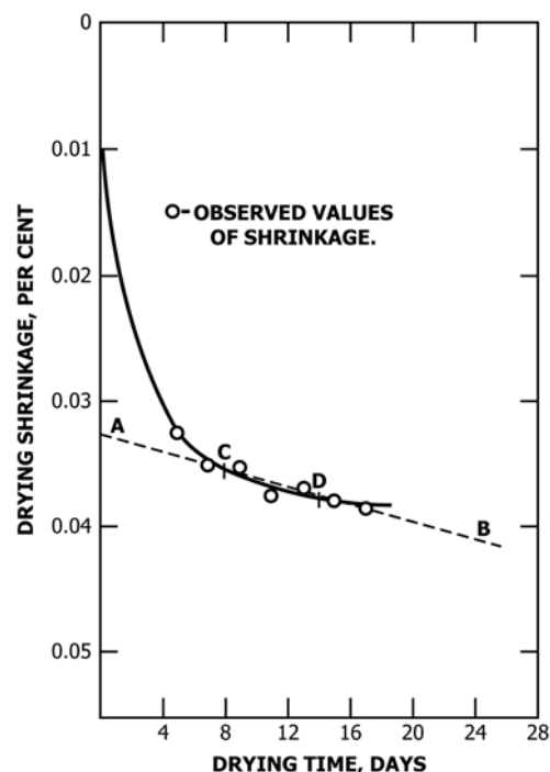
FIG. 3 Graphical Method of Determining Equilibrium Shrinkage
