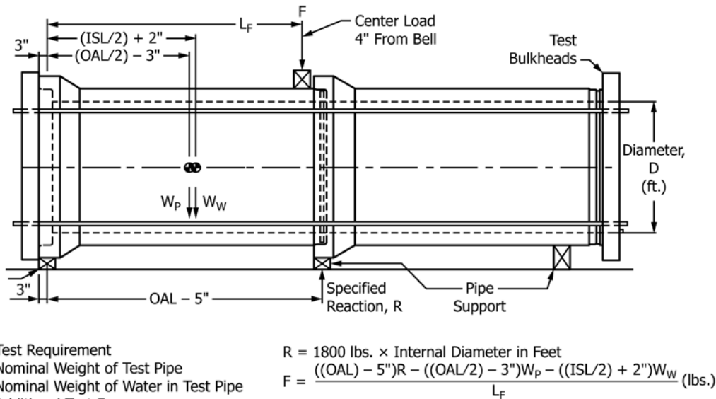
FIG. 11 Off-Center Hydrostatic Joint Test
