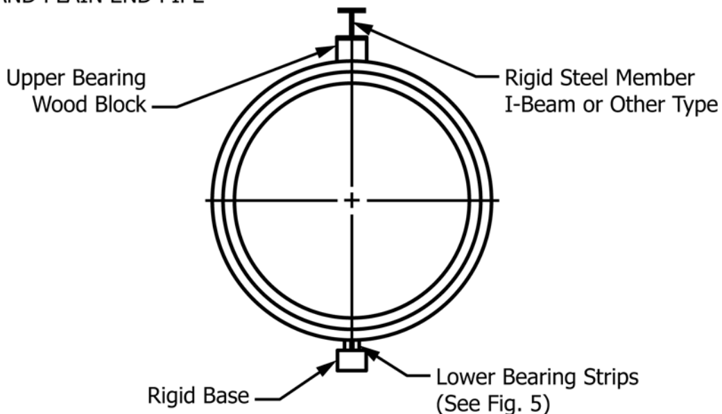
BELL OR SPIGOT AND PLAIN END PIPE
