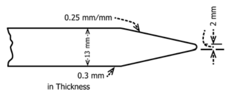
FIG. 6 Gage Leaf for Measuring Cracks
