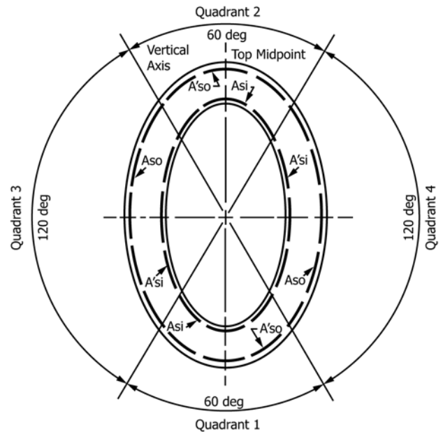
FIG. 2 Horizontal Elliptical Pipe
