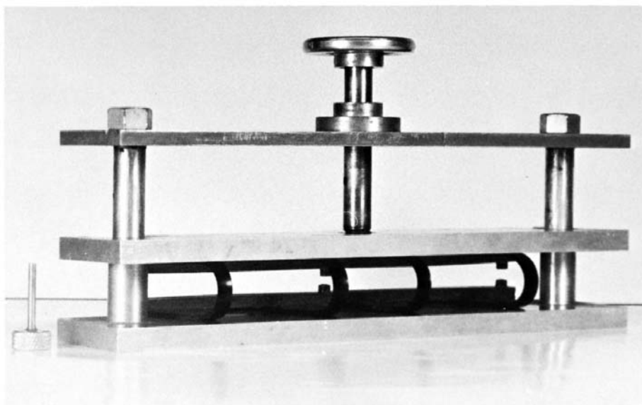
FIG. X1.1 Flexing Fixture for Low-Temperature Brittleness Test
